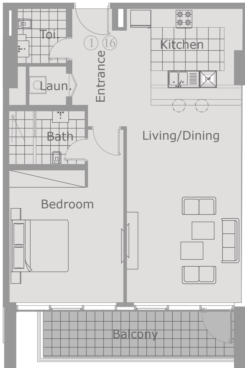
TOPAZ AVENUE 1 st Floor Layout 1 Bedroom
